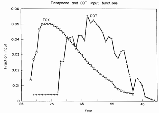
Fig. 5. Input functions (fraction of total input versus time) for toxaphene and DDT, derived from their rates of accumulation in dated North American peat cores. Reprinted from Atmospheric Environment , vol. 20, R. Rapaport and S.J. Eisenreich, pp. 2367–2379, copyright (c) 1986, with permission from Pergamon Press Ltd., Headington Hill Hall, Oxford OX3 0BW, UK.
