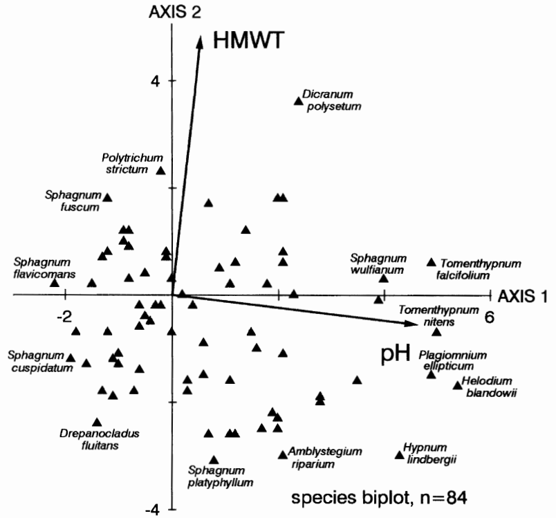
Fig. 2. Species-environment biplot, calculated by canonical correlation analysis. The environmental variables are represented by arrows. Eigenvalue for axis 1 = 0.55, for axis 2 = 0.39.
